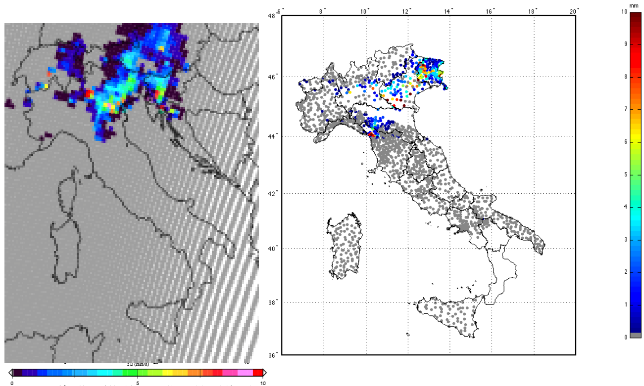
Figure. H02 precipitation map at 01:23 UTC (left) and raingauges hourly precipitation cumulated at 02:00 UTC (right) on July the 24 th 2011.
